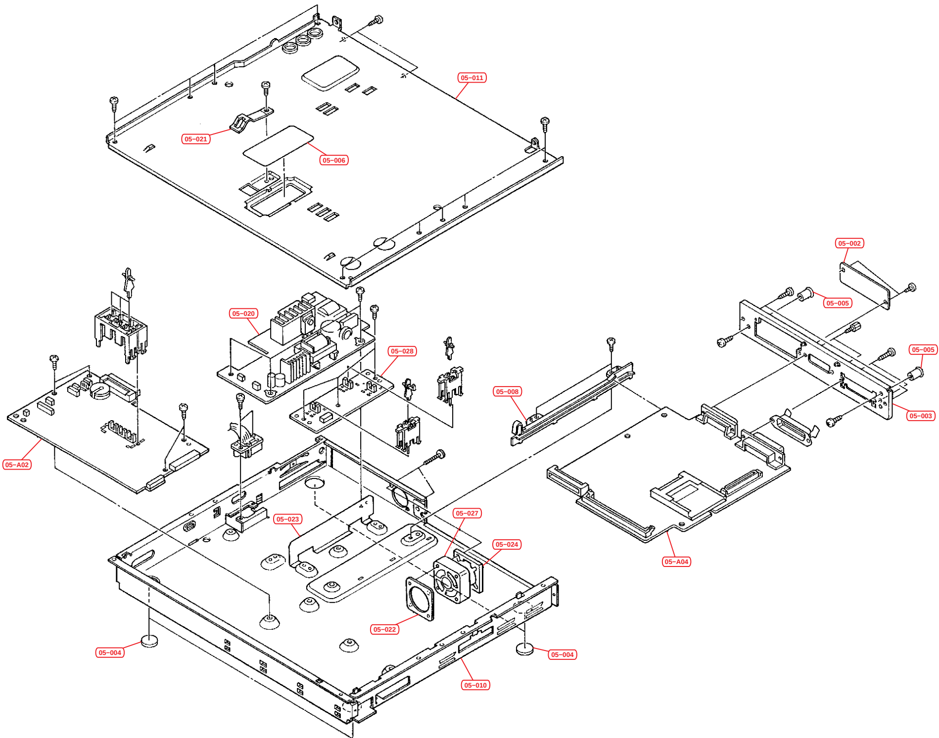
Fig.5 – Controller Unit
