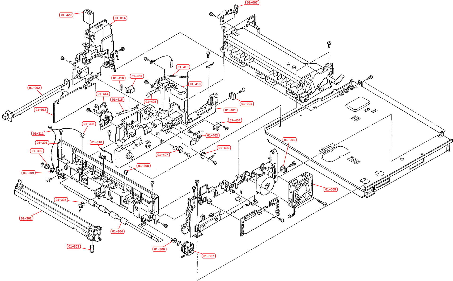
Fig.1 – Frame Unit
