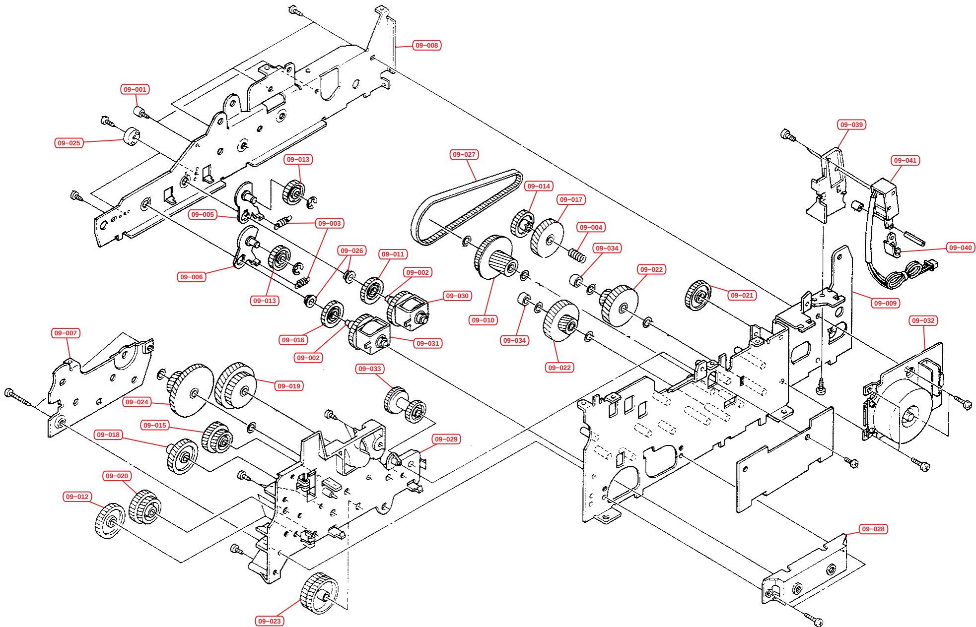
Fig.8 – Drive Unit
