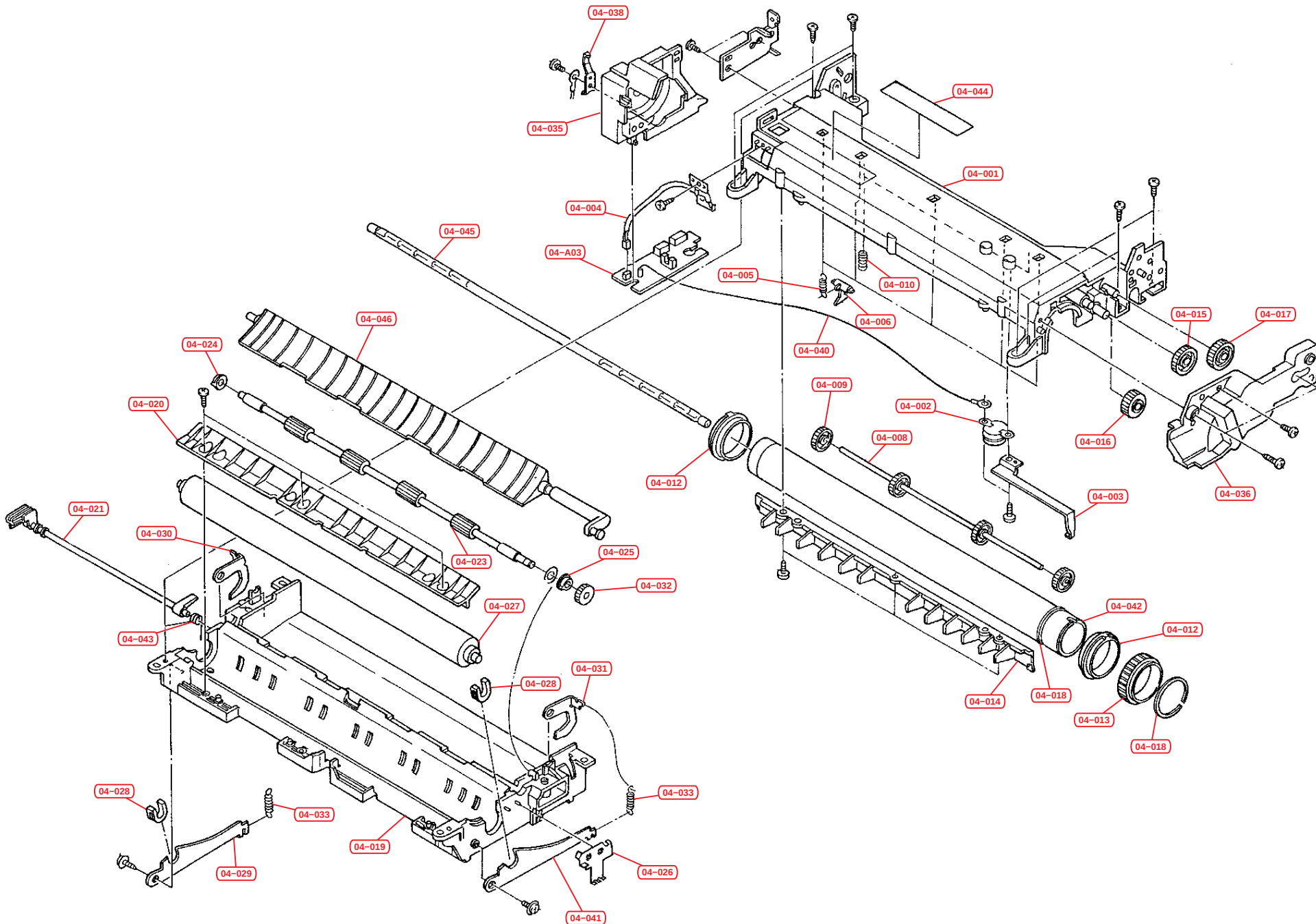
Fig.4 – Fuser Unit
